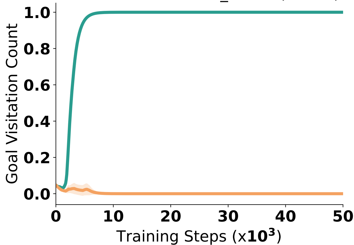
Gridworld-Bottleneck_Button(80.0%)
